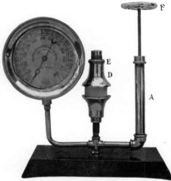
FIG. 1.—MACHINE WITH CEMENT RING IN POSITION READY FOR A TEST.
