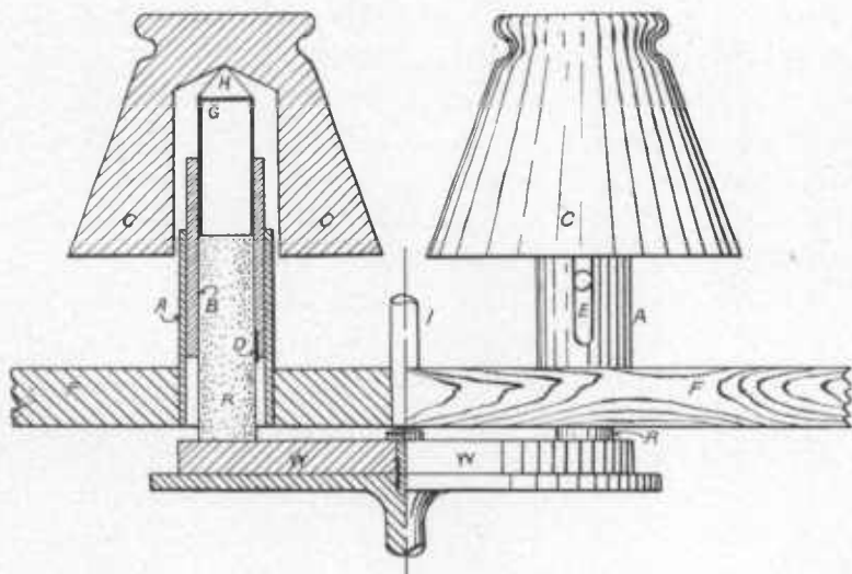
FIG. 18.—Sketch showing a half section and half elevation of machine for making wearing tests of stone and brick.
