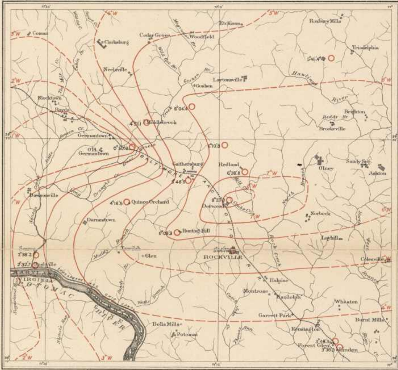
LINE OF EQUAL MAGNETIC DECLINATION IN NEIGHBORHOOD OF GAITHERSBURG, MD., FOR JAN. 1, 1900.
