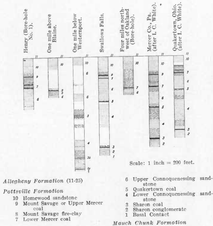
FIG. 21.—Columnar Sections of the Pottsville Formation.
