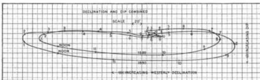
FIG. 3. Diurnal variation of curve of declination and inclination at Washington, D. C. (1889-1890).
