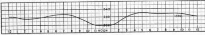
FIG. 5.—The diurnal variation of the vertical intensity at Washington, D. C. (1890).
