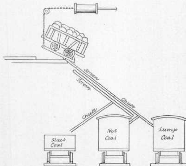
FIG. 38.—Sketch showing Main Tipple, Ocean No. 7, Consolidation Coal Company.
