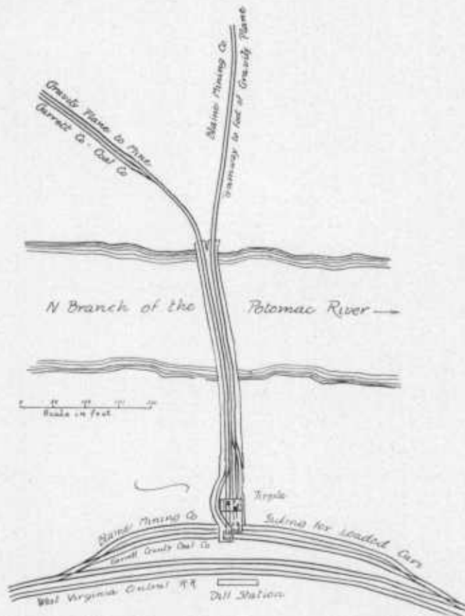
FIG. 53.—Tipples of the Blaine Mining Company and Garrett County Coal Company, at Dill.
