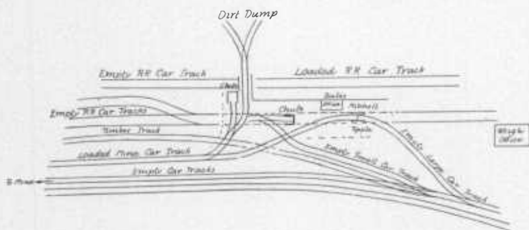
FIG. 47.—Sketch showing Tracks and Three-chute Tippie, Jackson Mine, American Coal Company.
