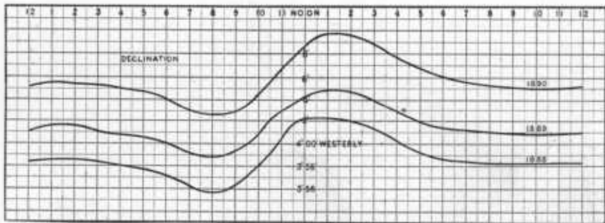
FIG. 1. Diurnal variation of the magnetic declination at Washington, D. C. (1888-90).
