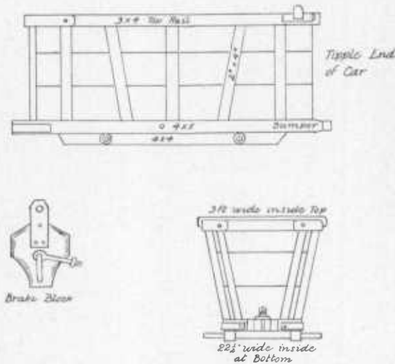
FIG. 35.—Sketch of Body of Mine Cars used by Consolidation Coal Company.
