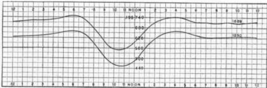
FIG. 4.—The diurnal variation of the horizontal intensity at Washington, D. C. (1889-1890).
