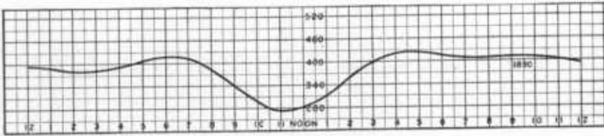
FIG. 6.—The diurnal variation of the total intensity at Washington, D. C. (1890).
